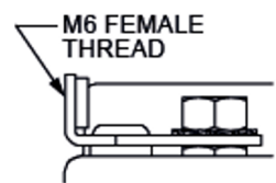
ODS-AGM16B LEFT POSITIVE FRONT FEMALE CONNECTION
